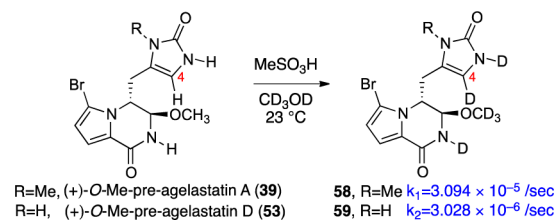
Scheme 14. Rate Constants for the Deuterium Incorporation at C4 of (+)-39 and (+)-53
