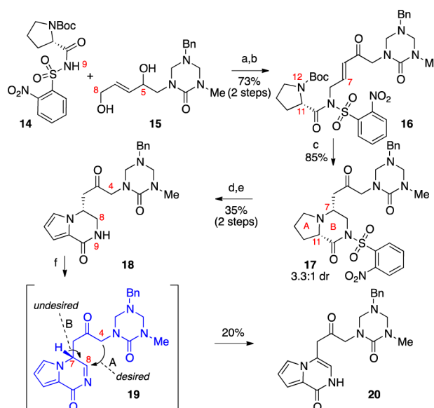
Scheme 3. Synthesis of Key Bicycle 18 and Attempted Oxidation–Cyclization a
