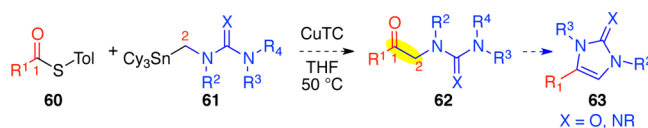
Scheme 15. Versatile Synthesis of Azaheterocycle 63
